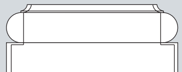
BSES-10 • 9 1/2" Top Width • 13 3/8" Base Width • 5 3/8" Height • To fit CLM TF-10
